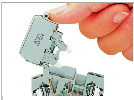
Fuse replacement:
