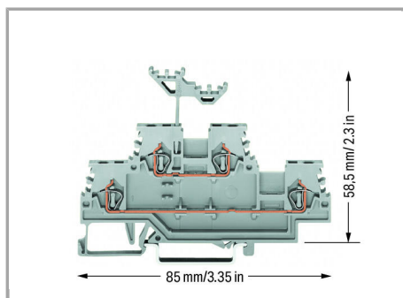
Double-deck marker carrier
