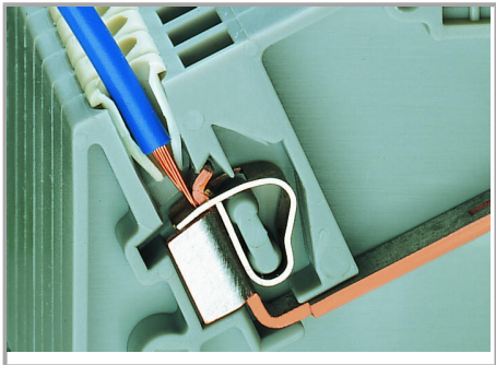
Insulation stop – prevents the conductor insulation from being pushed into the clamping unit (available for terminal blocks up to 4 mm²/12 AWG).
