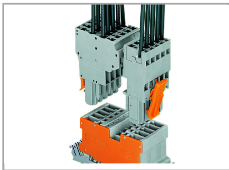
2-pin carrier terminal block with shield contact
