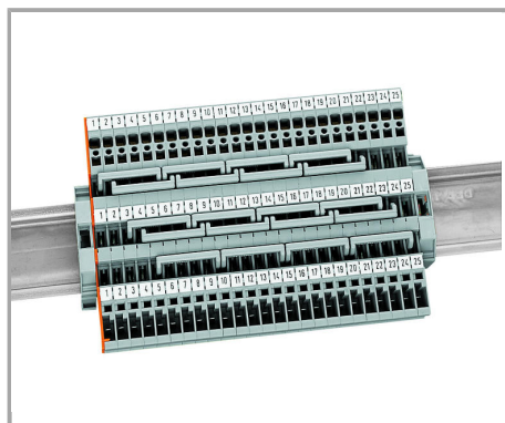
1-conductor/1-pin carrier terminal blocks with three jumper positions
