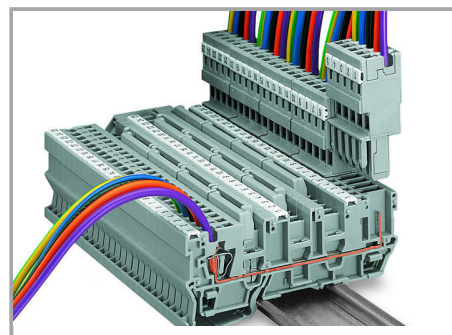
1-conductor/1-pin carrier terminal block with three jumper positions
