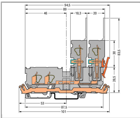
Female plug secured with locking lever on the terminal block side.
