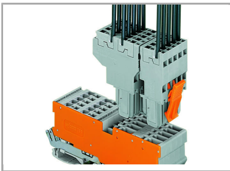
2-conductor/2-pin carrier terminal block with shield contact
