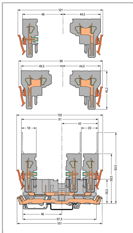
Carrier terminal block with shield contact
