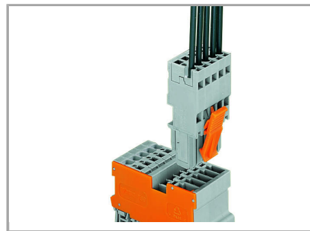
1-conductor/1-pin carrier terminal block
