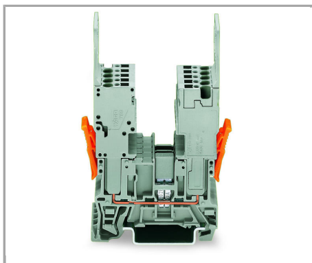
1-conductor female plugs
