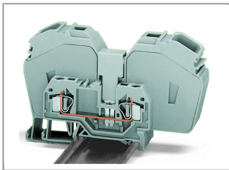
Commoning with step-down jumper (283-414) from 285 Series (35 mm²/2 AWG) to 281 Series terminal blocks (4 mm²/12 AWG).
