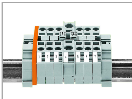
Commoning from 10 mm²/8 AWG (284 Series) to 6 mm²/10 AWG (282 Series) rail-mount terminal blocks via step-down jumpers.
