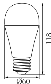
● A60 LED N 15W E27
