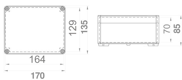
Krabice SolidBOX IP65 / Sealed box IP65 - Obj.č. / Item 68120 / 68121
