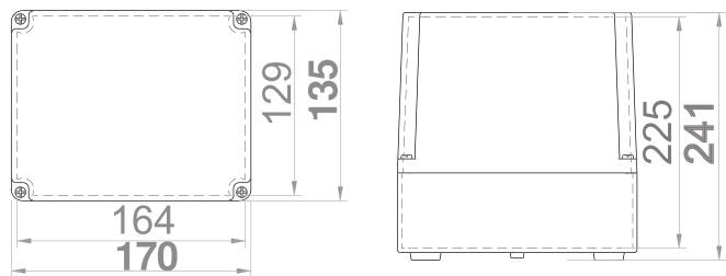
Krabice SolidBOX IP65 / Sealed box IP65 - Obj.č. / Item 68100 / 68101
