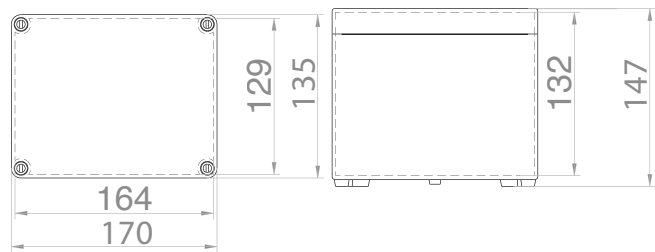
Krabice SolidBOX IP65 / Sealed box IP65 - Obj.č. / Item 68090
