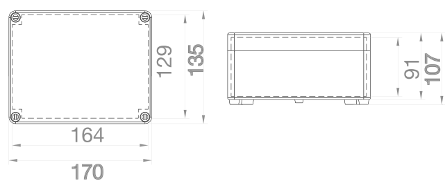
Krabice SolidBOX IP65 / Sealed box IP65 - Obj.č. / Item 68120 / 68121
