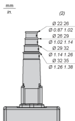
(2) Internal Ø (mm/in.)
