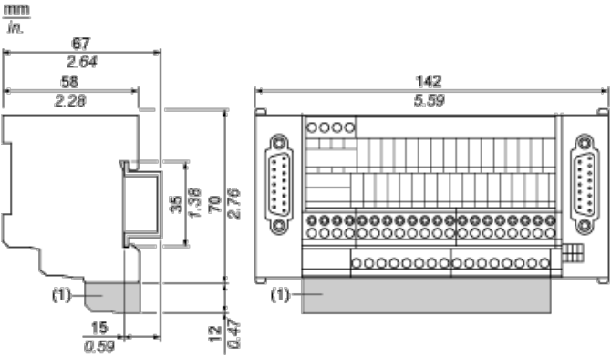
(1) ABE7BV10 / ABE7BV20
