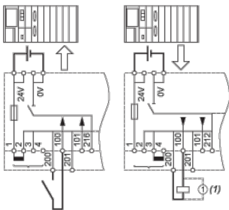
(1) Inductive load
