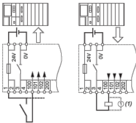
(1) Inductive load
