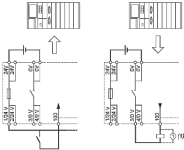
(1) Inductive load
