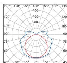
DUST EVG PC 2 × 18W
