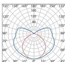
DUST EVG PC 1 × 18W
