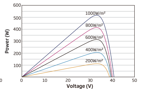
P-V CURVES OF PV MODULE (520W)
