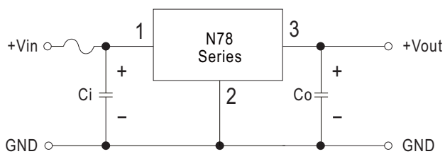
Positive output application circuit
