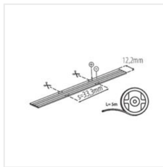
LCOB2L 28W/M24IP65-CW
