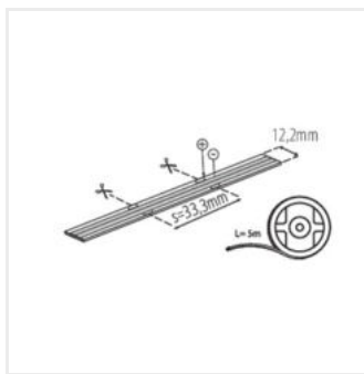
LCOB2L 28W/M24IP65-NW
