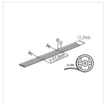
LCOB2L 28W/M24IP65-WW
