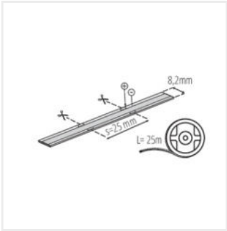
LCOBB 3W/M 12 IP65-CW
