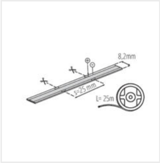
LCOBB 3W/M 12 IP65-WW
