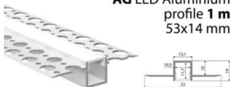
AG LED Aluminium profile 1 m 53x14 mm
