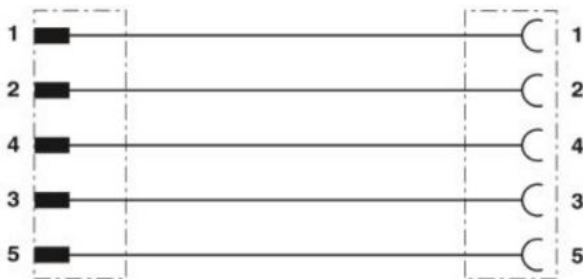
Pin assignment between M12-plug and M12-jack
