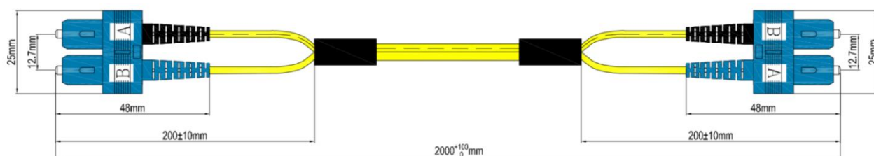
Dimensional drawing
