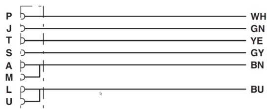
Pin assignment M16 jack
