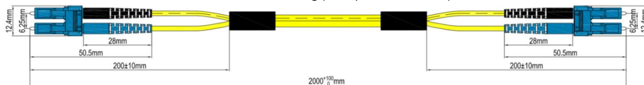
Dimensional drawing (example of 29033902)
