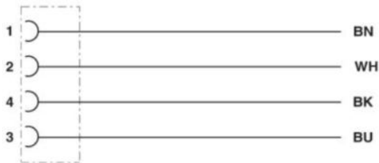
Circuit drawing
