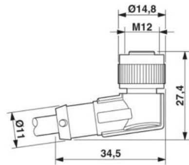
Jack M12 x 1, angled
