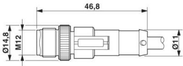
Plug M12 x 1, straight
