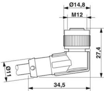
Jack M12 x 1, angled
