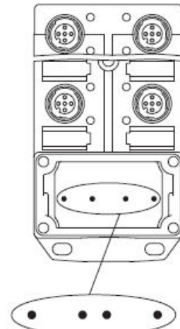
Potential separated. Potential order: U_{N1} = slots 1, 3 and U_{N2} = slots 2, 4
