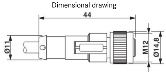
Jack M12 x 1, straight
