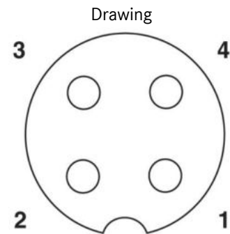
Pin assignment M12-jack, 4-pol, A-coding
