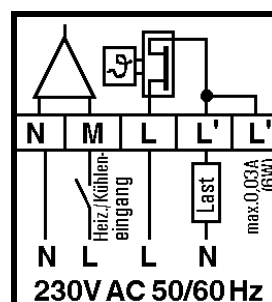
HK07 Raumthermostat Premium
