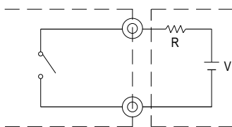
Fig 2.2 Internal circuit of AC OK (Battery Low)
