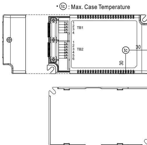
Terminal Pin No. Assignment(TB2)
