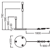
DECOR STICK FLOOR 3XE27 DIM DG
