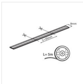
LCOB 10,5W/M 24
