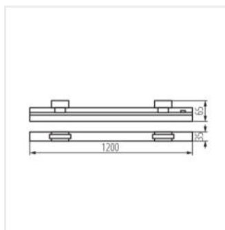
LTL-E 24W-120-CCT-W
