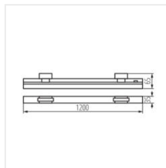
LTL-E 24W-120-CCT-B
