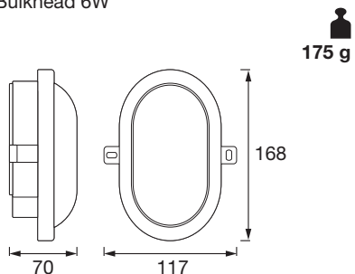
LED Bulkhead 6W
