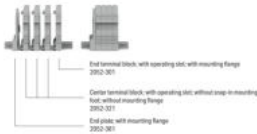
Examples of a 4 pole terminal block, with operating slot, with mounting flange
