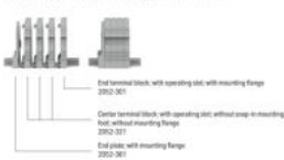
Example of a 4-pole terminal strip with operating slot, with mounting flange
