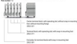
Example of a 5-pole terminal strip with operating slot, with snap-in-mounting flange
