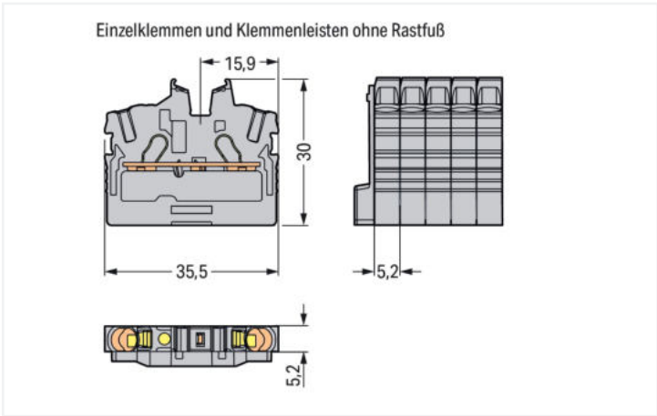
Through terminal block, 2052 Series, blue
