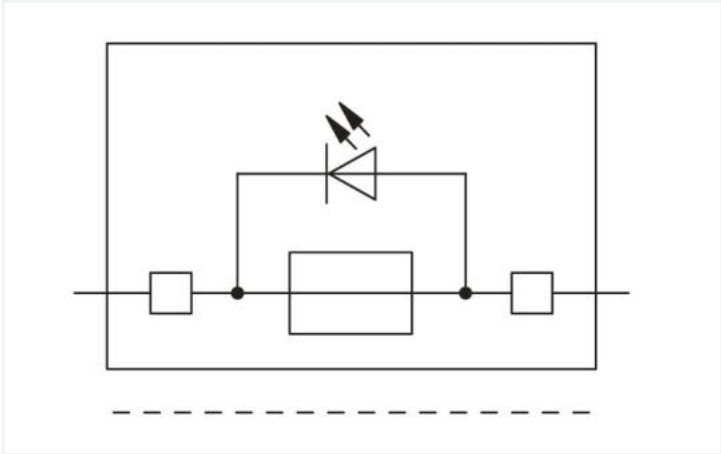
Fuse terminal block, 2202 Series, blue
