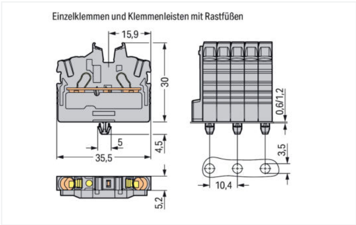
Through terminal block, 2052 Series, green-yellow
