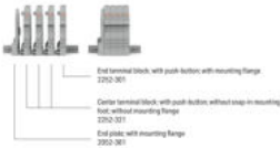
Example of a 4 pole terminal block with push buttons with mounting flange
