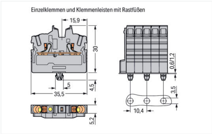
Through terminal block, 2252 Series, gray
