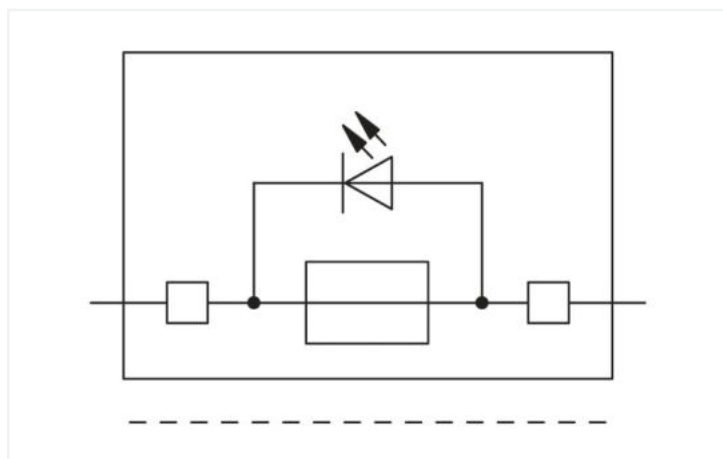
Fuse terminal block, 2002 Series, blue
