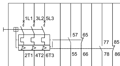
Trip Signalling Block TSBE
