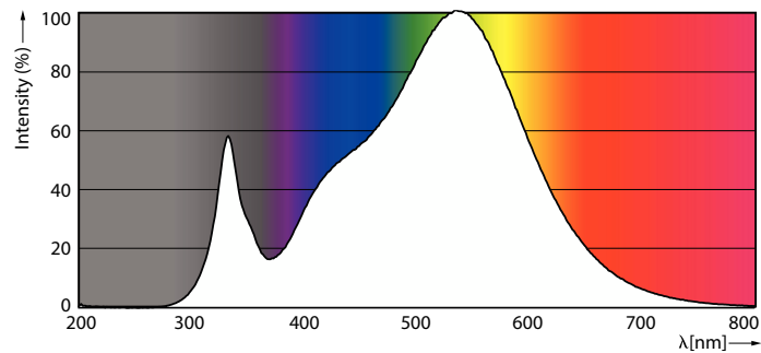
Spectral Power Distribution Colour - CorePro LEDtube 1500mm UO 25.9W 830 T8
