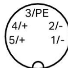
7/8" plug
