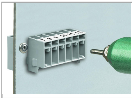
Mounting with 3 mm Ø blind rivets
